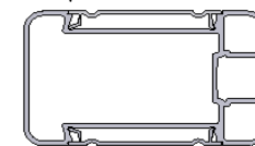
Montant 100x60 + clips
